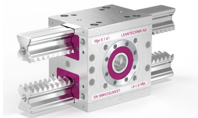
lifgo® double SVZ
