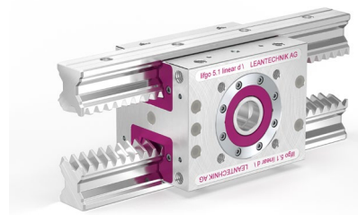
lifgo® linear double SVZ
