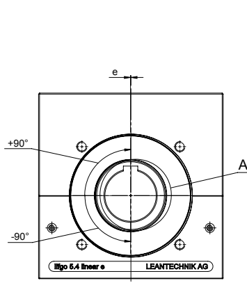
lifgo® eccentric
